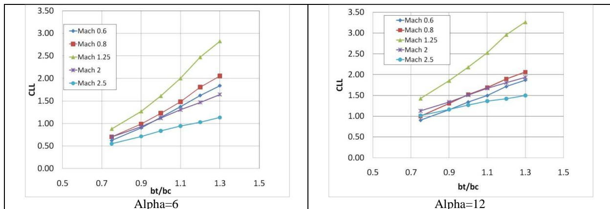
Figure 13. Induced Rolling Moment for \delta_y=10^\circ (constant area)
