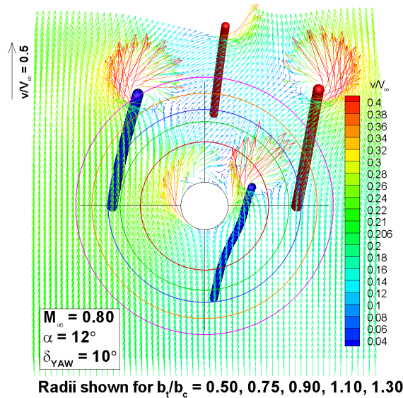
Figure 12. Yaw Control Velocity Maps
