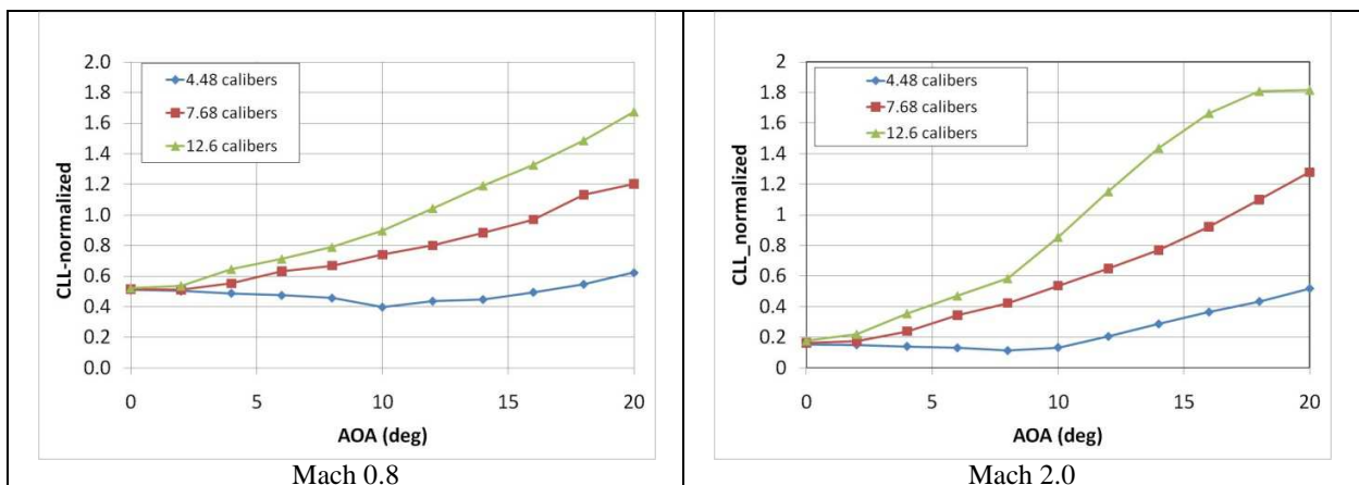
Figure 20. Impact of fin placement on roll authority, \delta_\gamma=5^\circ
