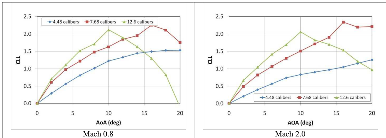
Figure 22. Impact of Fin Placement on Yaw Induced Roll, \delta_\gamma=10^\circ
