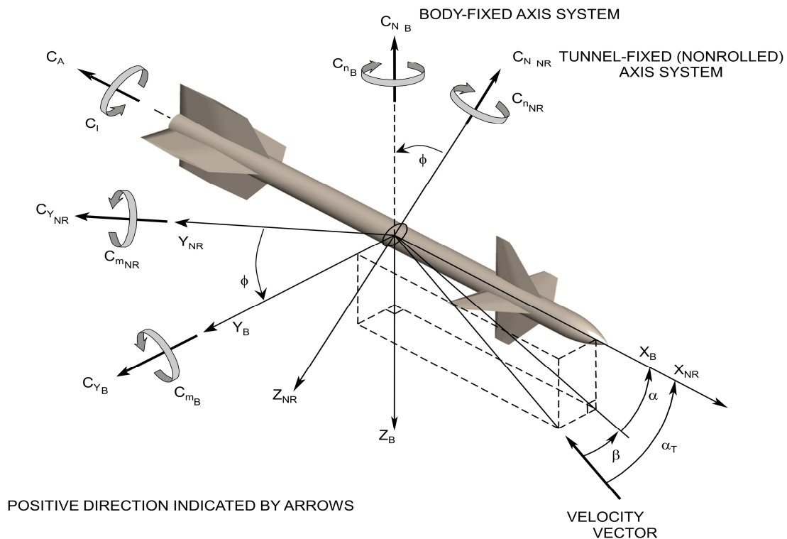
Figure 5. Sign Convention
