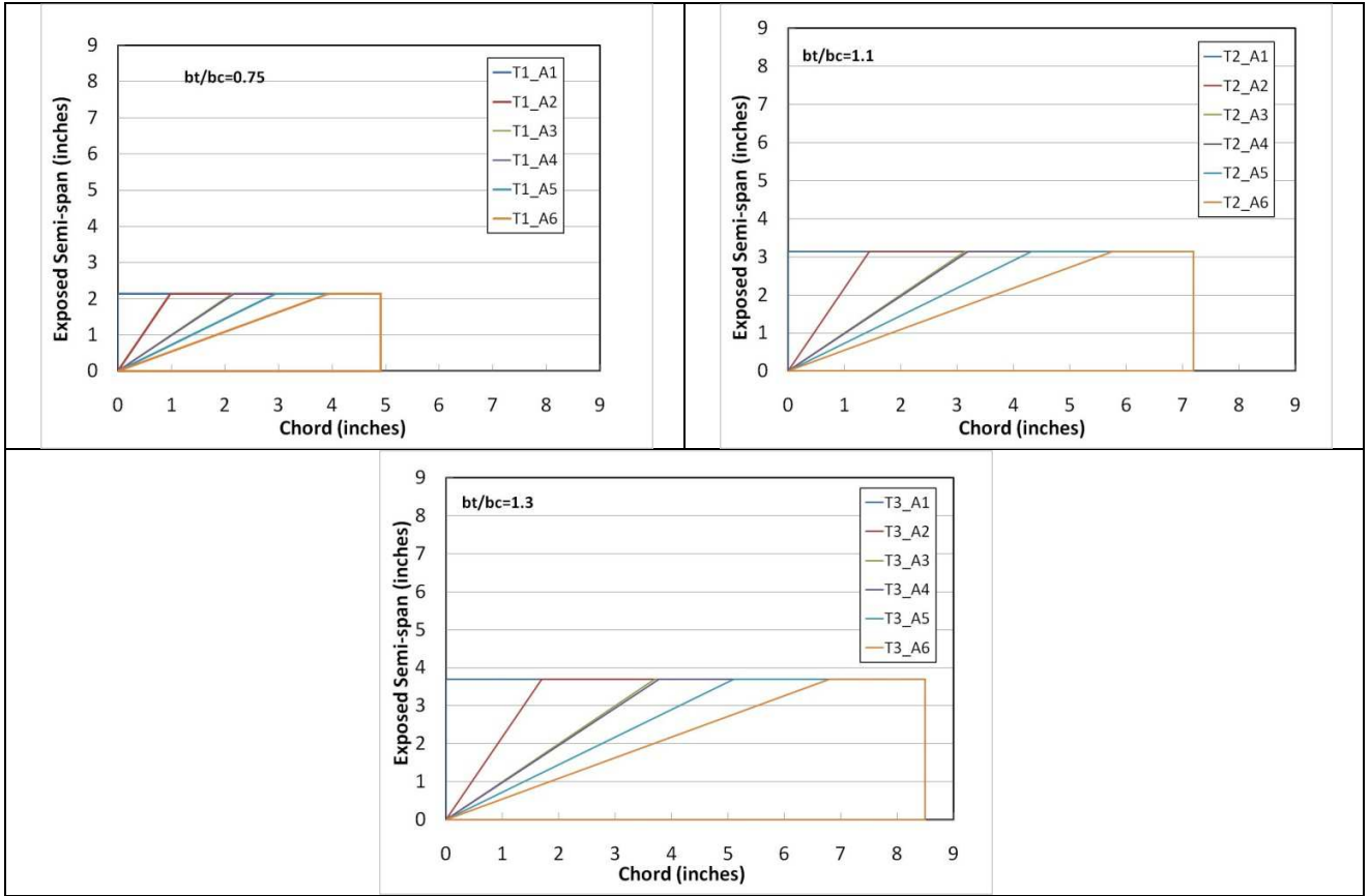
Figure 15. Tail Geometries for Varying Area
