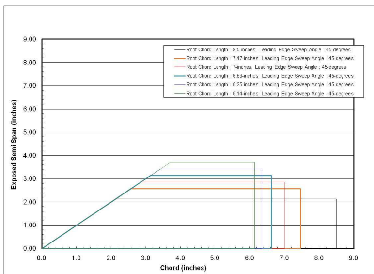
Figure 7. Tail Configurations for a Constant Area
