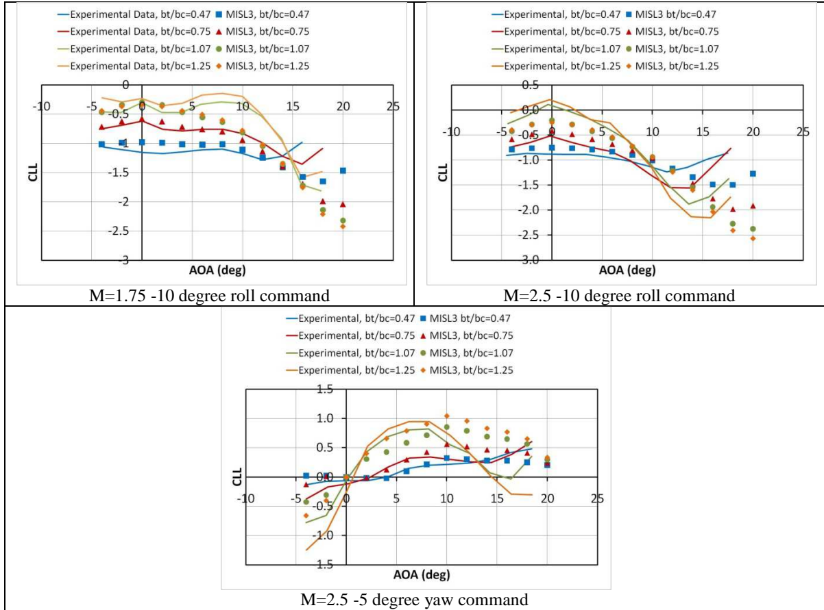
Figure 6. MISL3 comparison with Blair data
